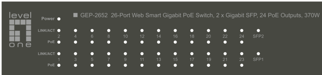
Figure 2 - LED Indicator
