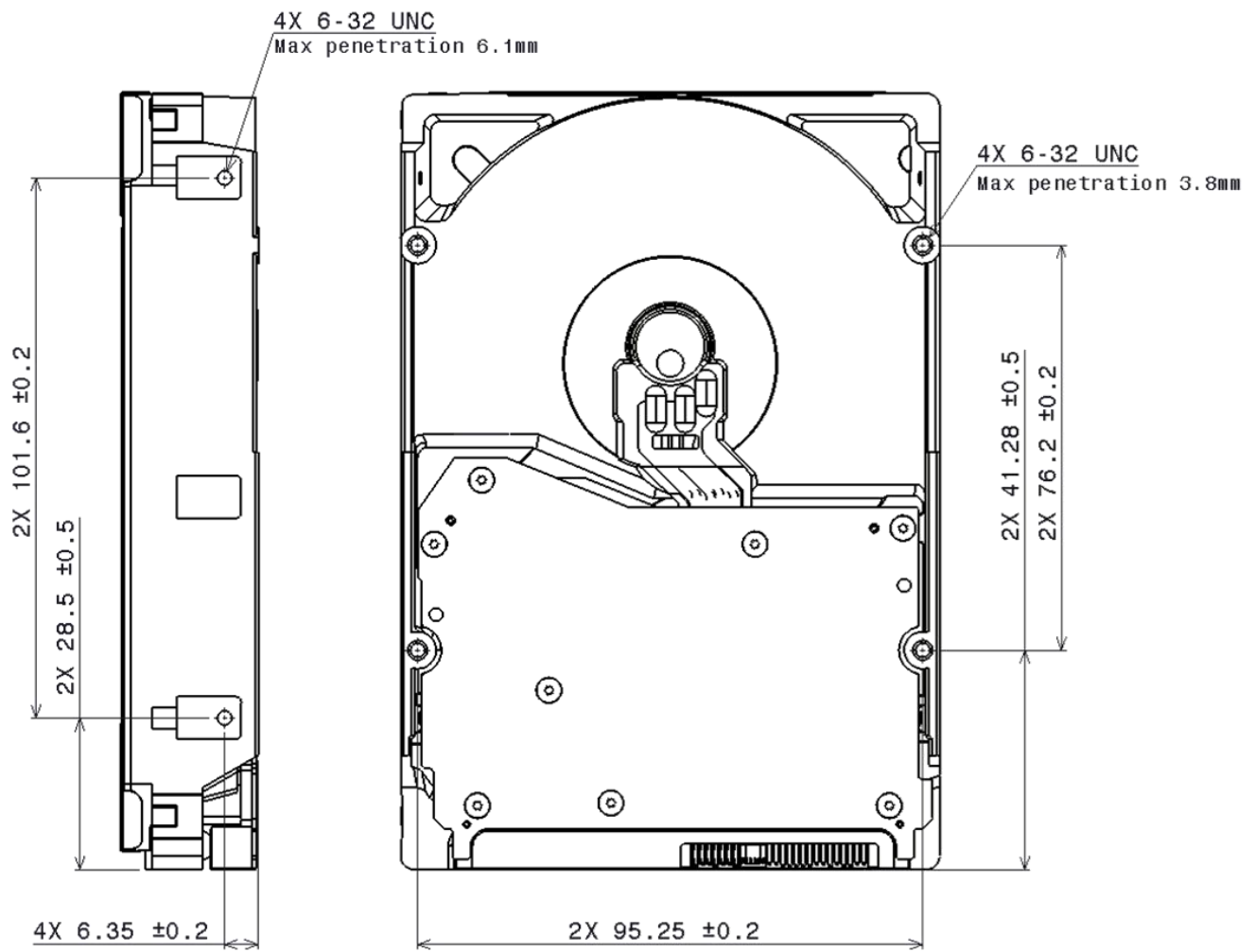
Figure 7 Bottom and side views with mounting hole locations All dimensions in the above figure are in millimeters.
