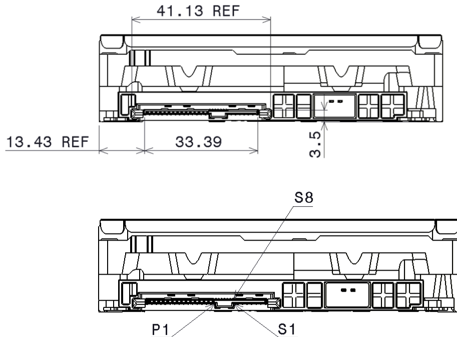
Figure 9 Connector locations
