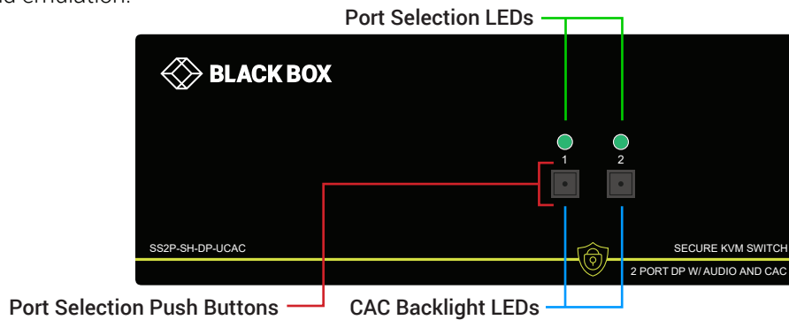
Figure 4-1: SS2P-SH-DP-UCAC Front panel
