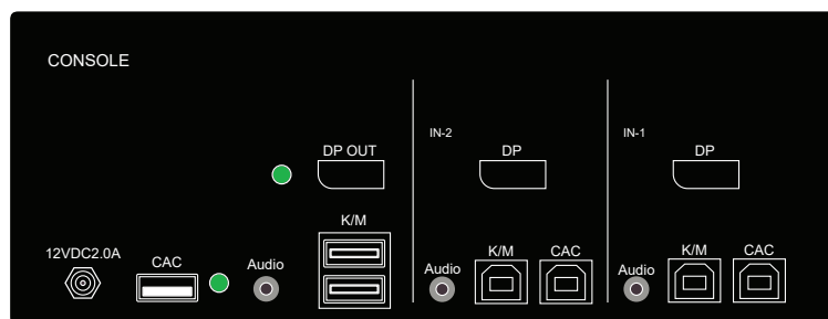
Figure 4-2: SS2P-SH-DP-UCAC Rear panel
