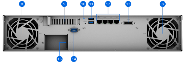
Rear (RS1221RP+)
