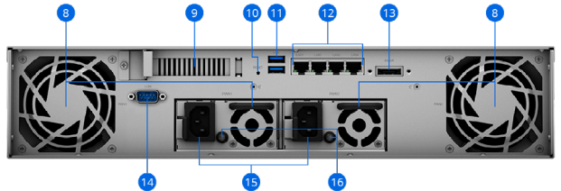
Rear (RS1221RP+)
