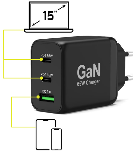
USB-C and USB-A ports allowing to charge one laptop and two additional devices Ports USB-C et USB-A permettant de charger un ordinateur portable et 2 appareils supplémentaires
